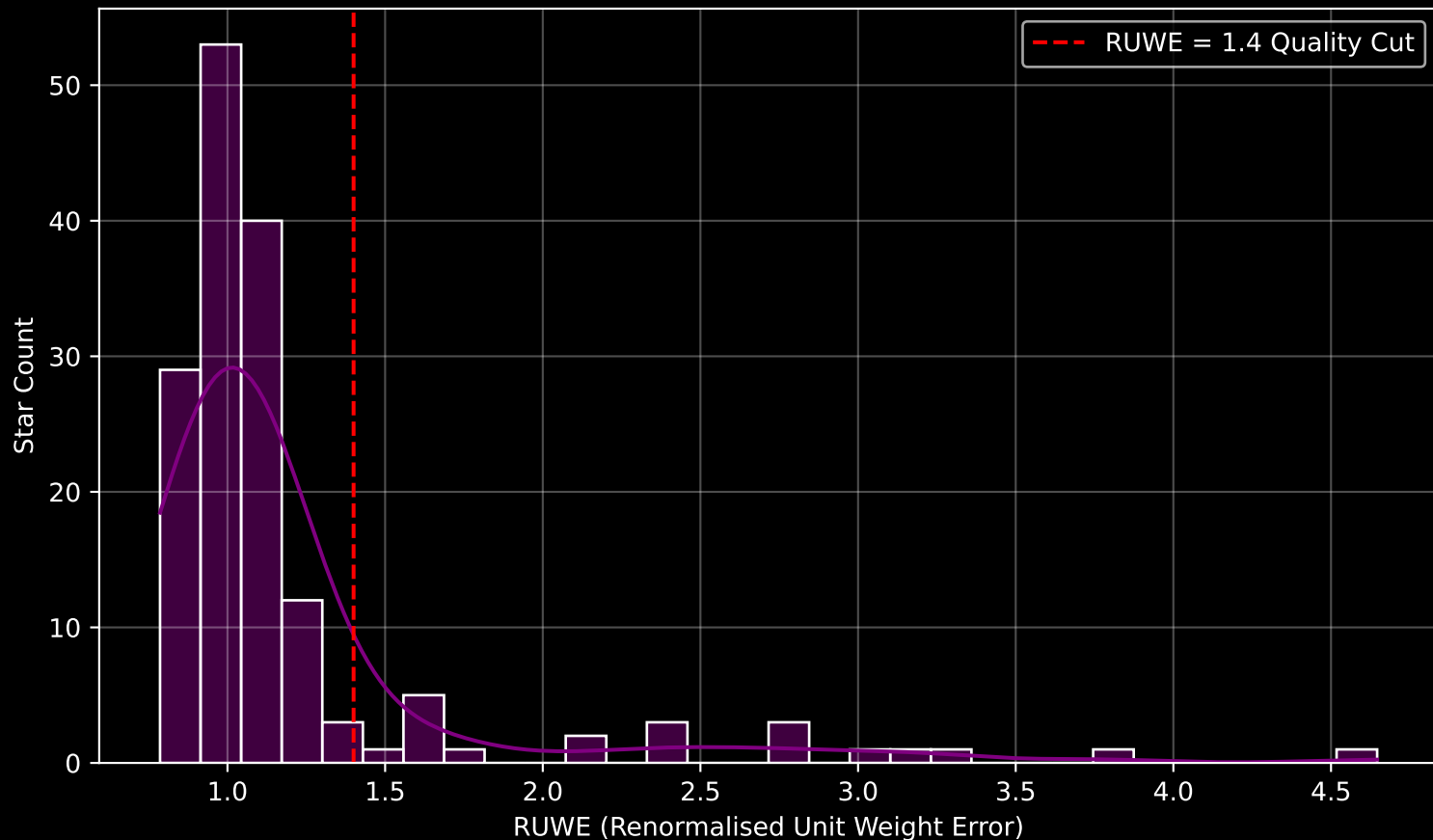
GAPOGEE DR17 Field [283-22-O_TESS] RUWE Distribution (n= 157)
