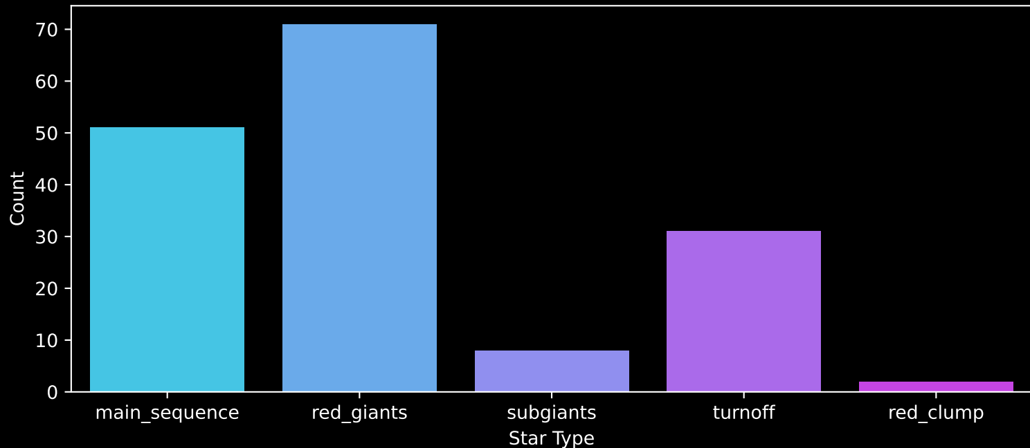
APOGEE DR17 Field: [283-22-O_TESS] Count plot of Star Type
